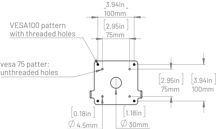
Vesa pattern details
