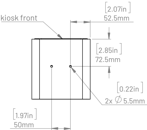
counter top mouting hole pattern
